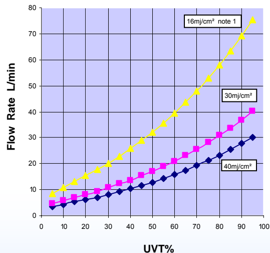
UVD320E Performance Curves note 2
